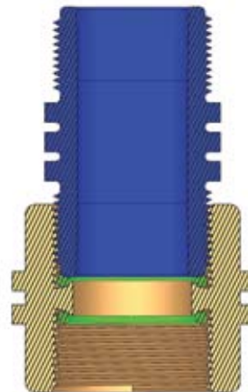
Seal on female thread O-ring
