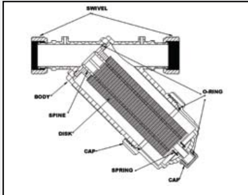
2" swivel disk filter
