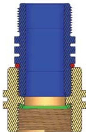
Seal on male thread O-ring
