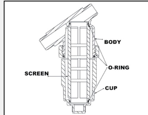
1" m/m screen filter
